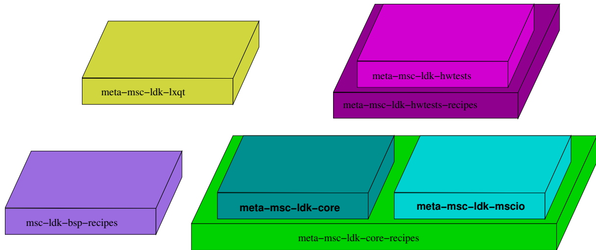
Figure 4.1. – MSC-LDK Layers
