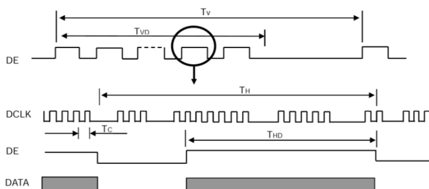
INPUT SIGNAL TIMING DIAGRAM
