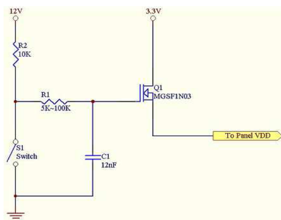
Test circuit
