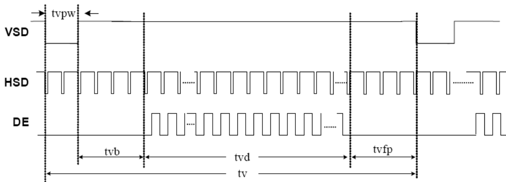
Vertical timing
