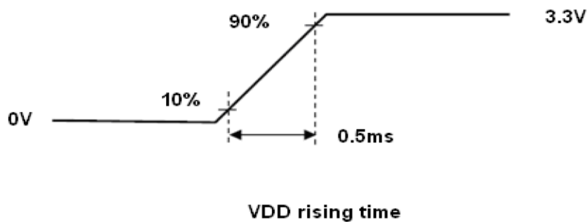
Figure 9 VDD rising time
