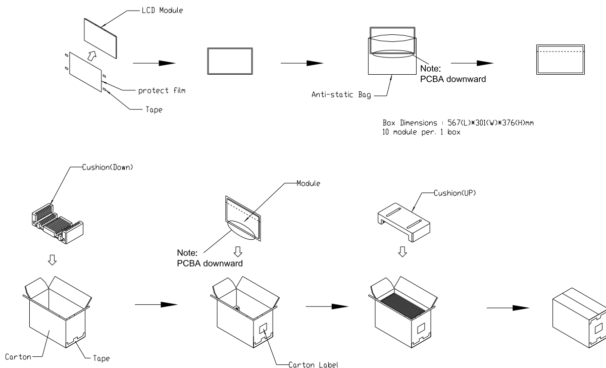
Figure. 8-1 Packing method
