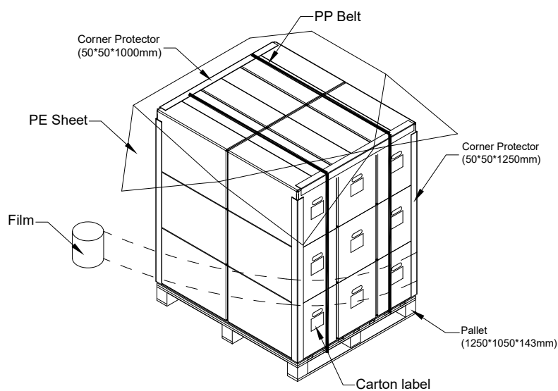
Figure. 9-2 Packing method
