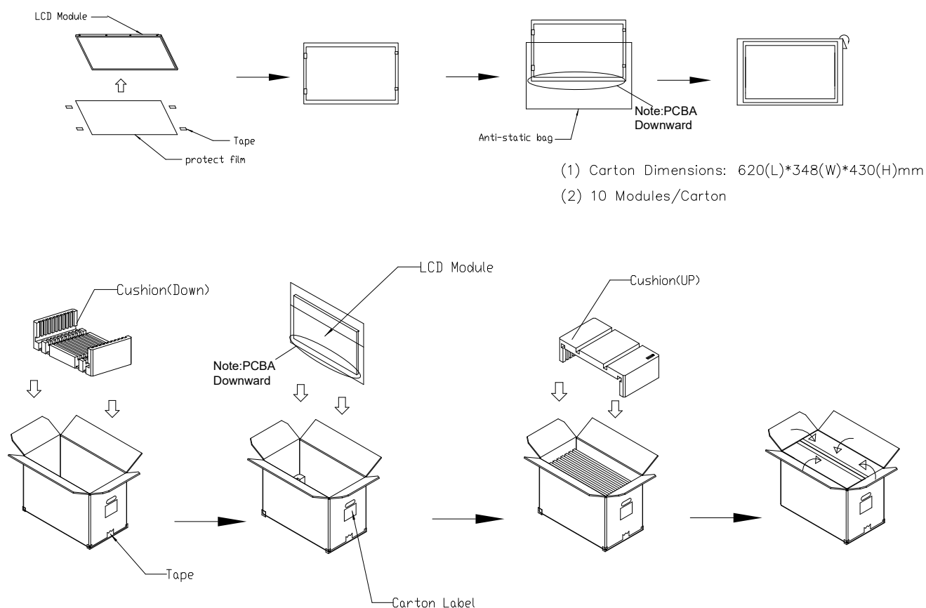
Figure. 9-1 Packing method
