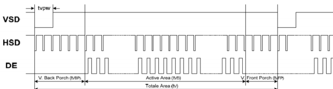
Vertical Input Timing
