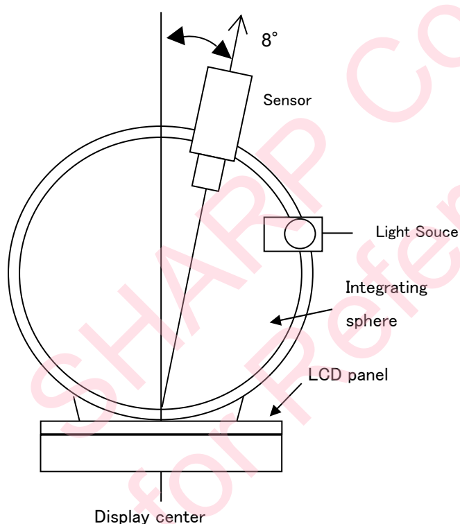
Figure 7-2 Contrast ratio, Reflection ratio, Panel chromaticity
