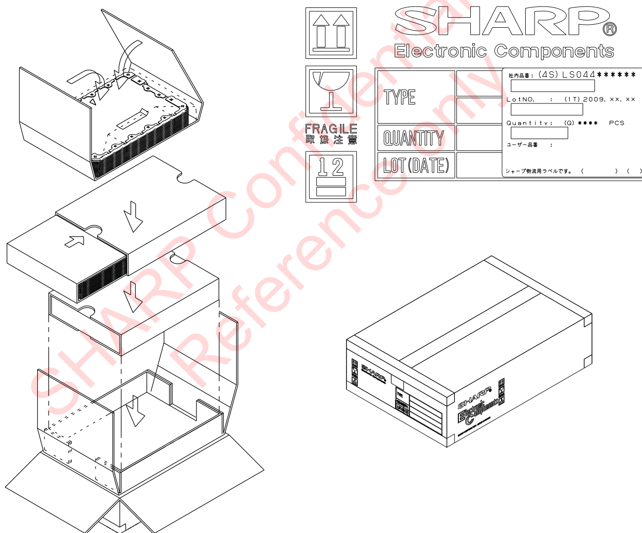
Figure. 12-1 Packaging Form
