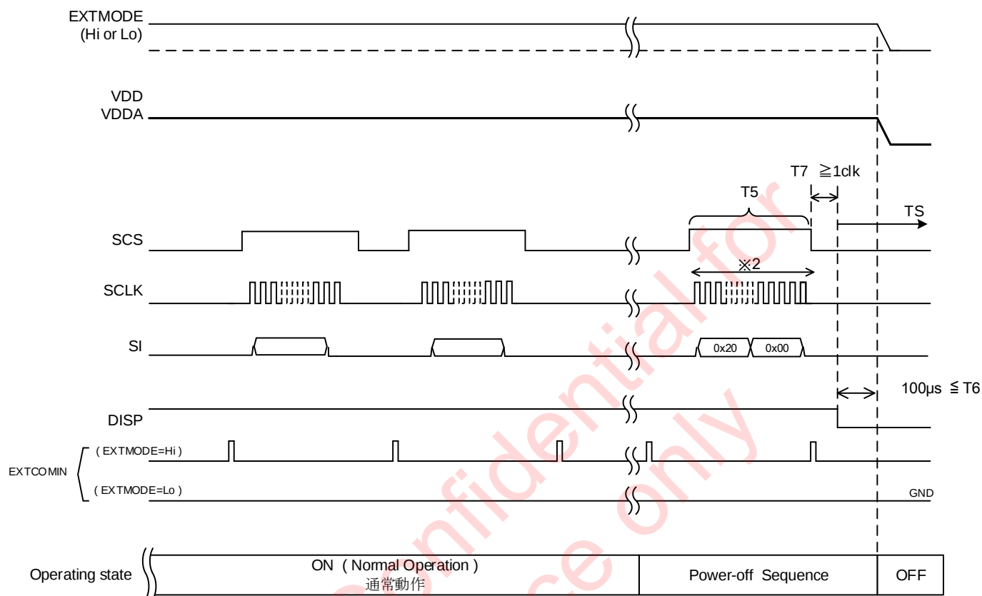
Figure 6-2 Power supply sequence
