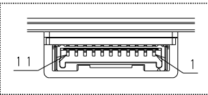
CN2/3 detail
