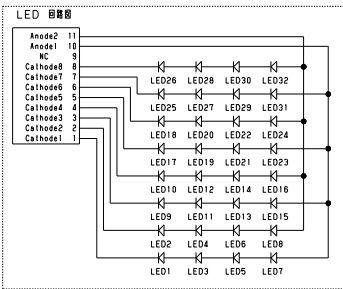
CN2/3 (LED Connector)
