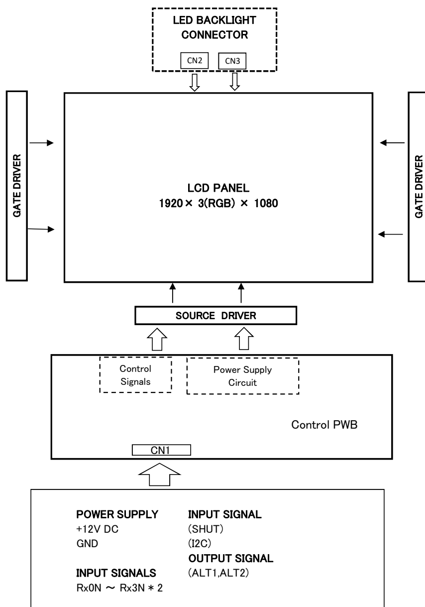
Fig.1 Block Diagram (LCD Module)
