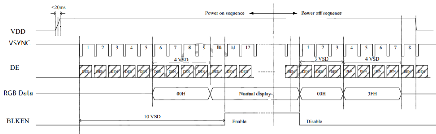
Figure 5.3.1 Power on/off sequence
