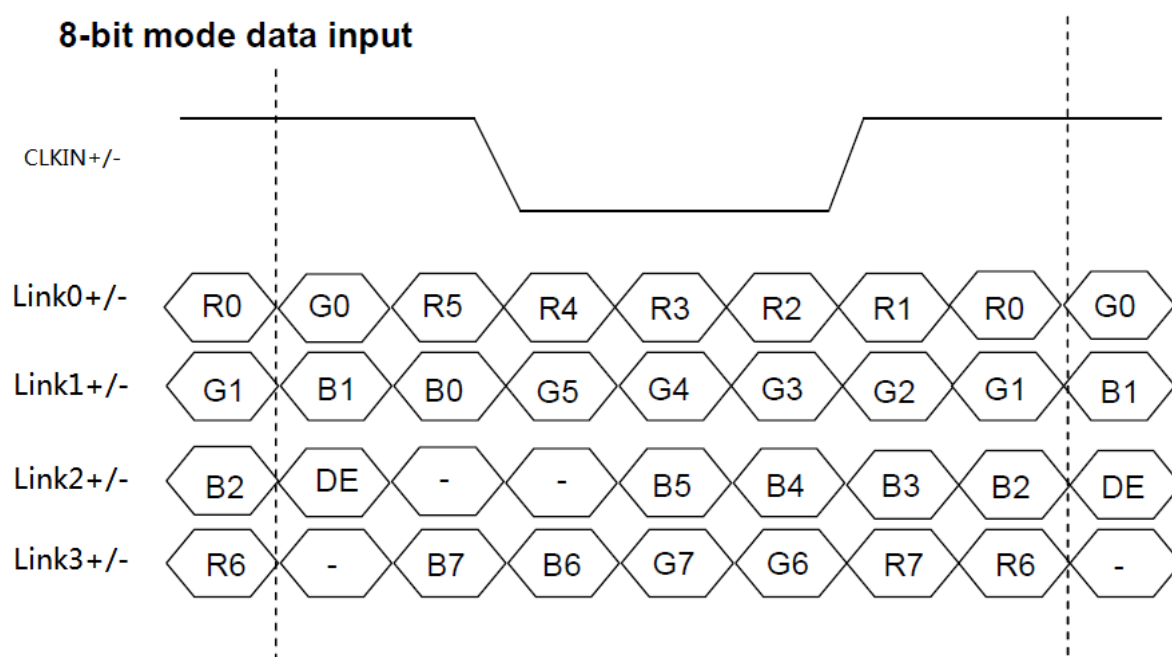
Figure 6.5.1 LVDS 8bit(Mode=H)
