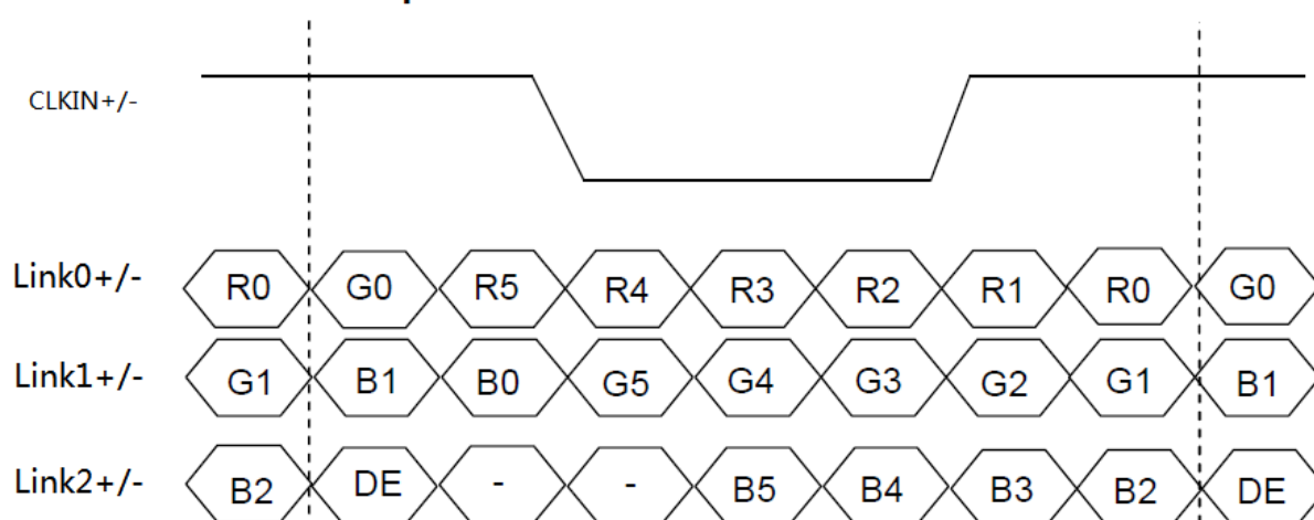
Figure 6.5.2 LVDS 6bit(Mode=L)
