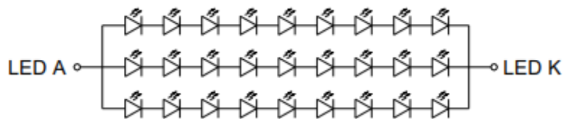
LED CIRCUIT
