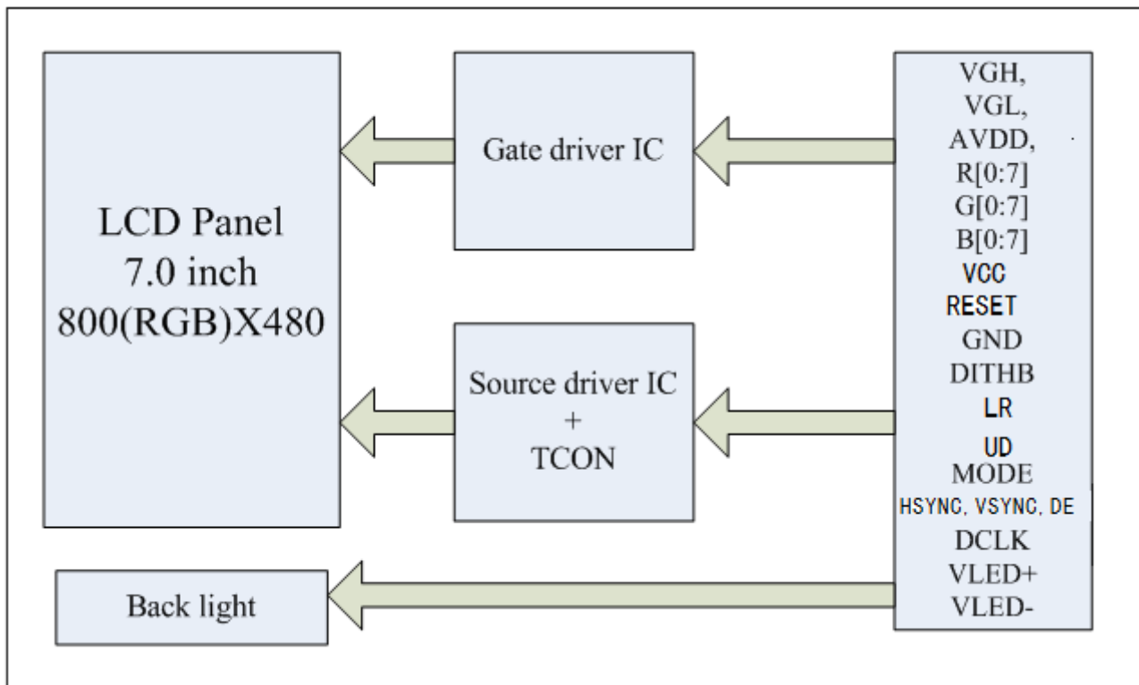
Figure 5.5.1 LCD Module Block Diagram
