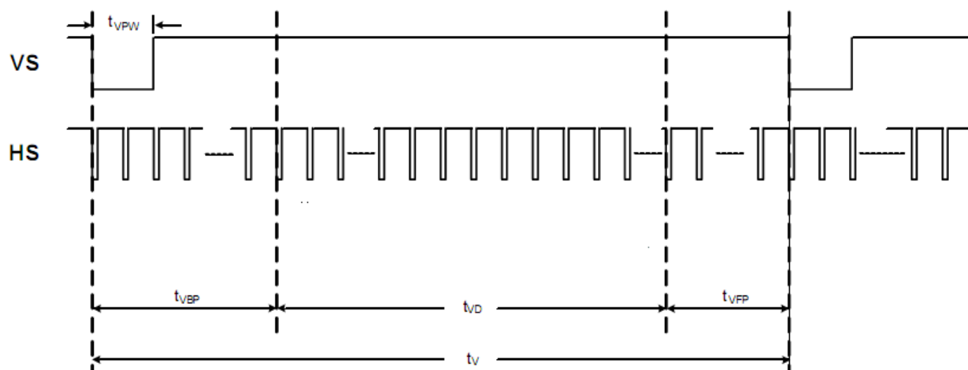
Figure 6.3 Input timing
