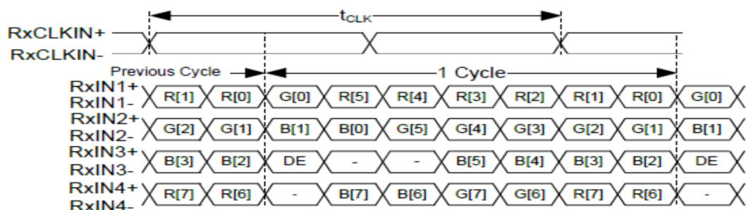
Figure 6.3. Data Input Timing Diagram Under DE Mode
