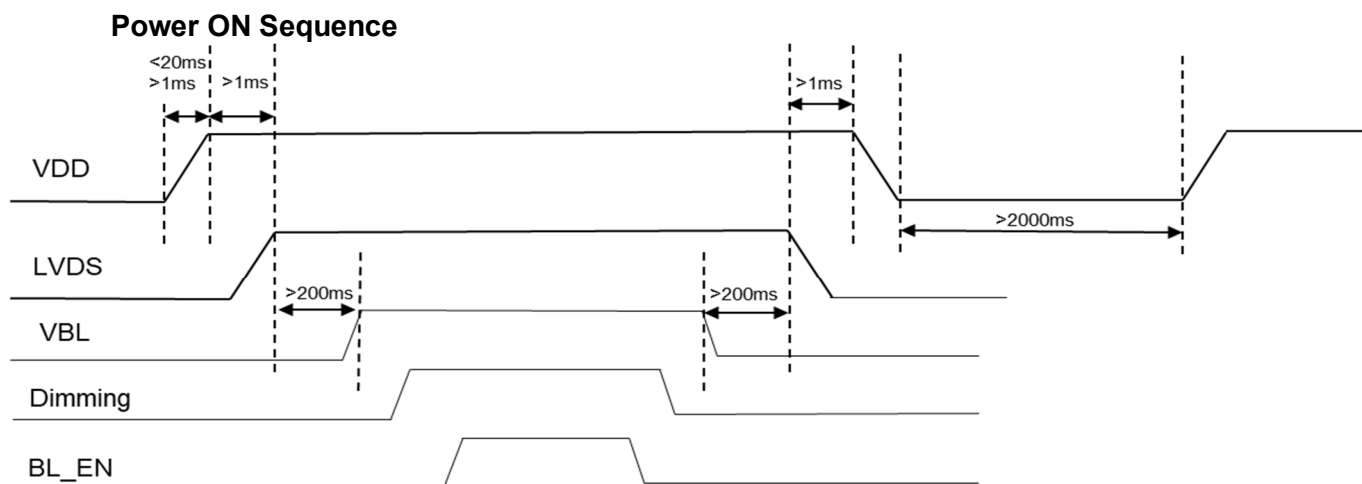
Figure 5.3.1Power on sequence
