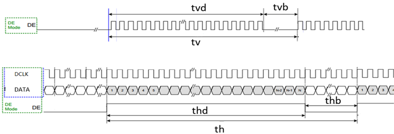
6.2 Data Input Timing Diagram Under DE Mode
