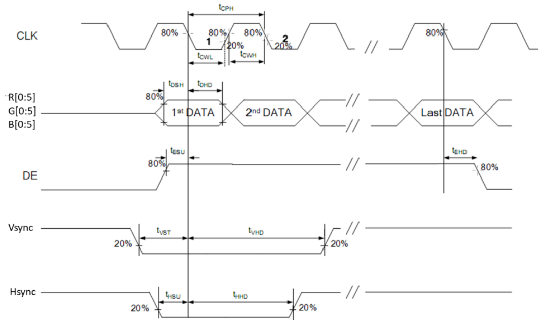
Figure 6.1.1 Clock and Data Input Timing Diagram
