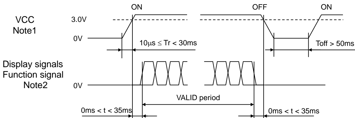
Figure 5.5.1 LCD on/off
