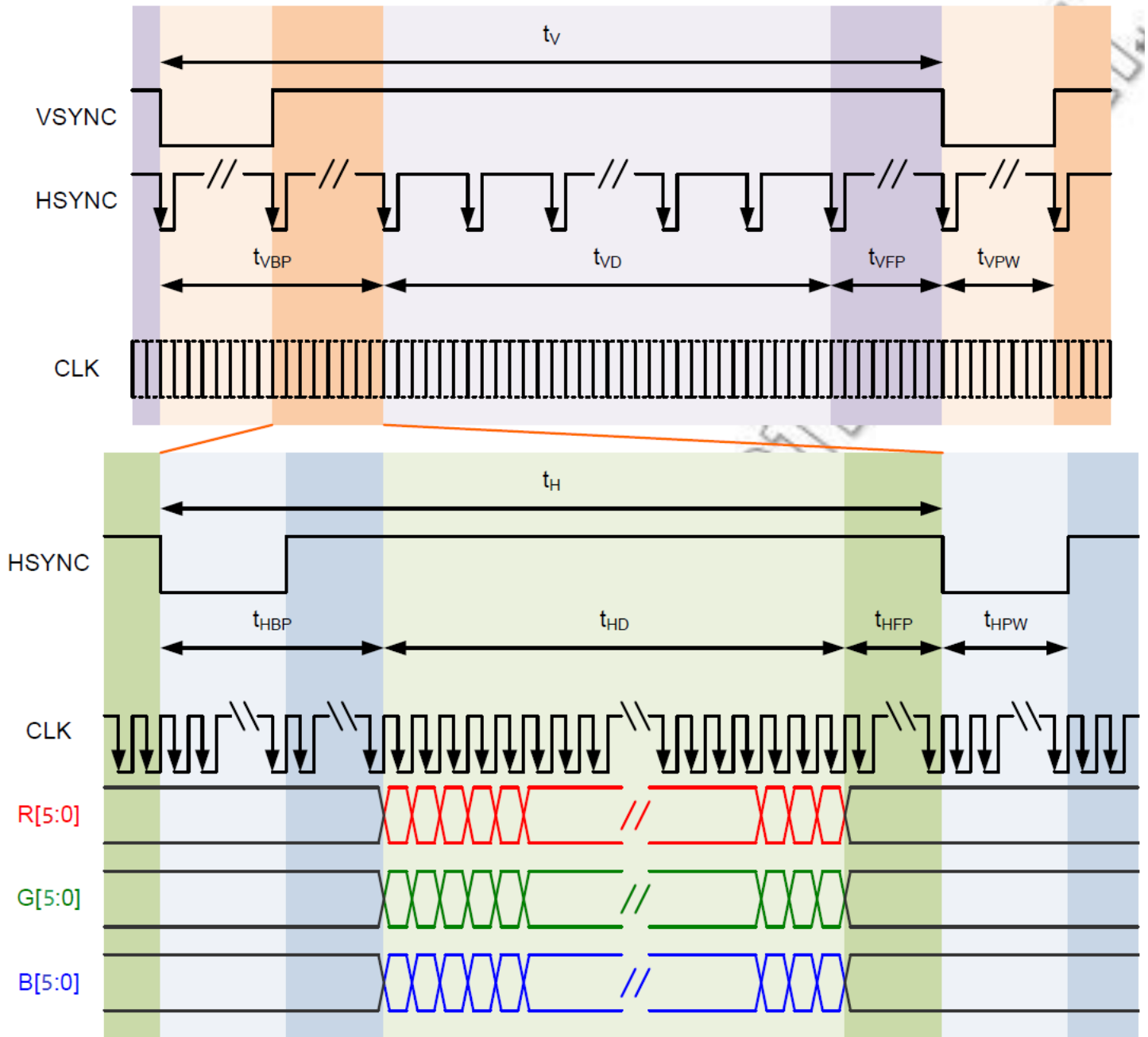
Figure 6.3.1 Data Input Timing Diagram Under SYNC Mode
