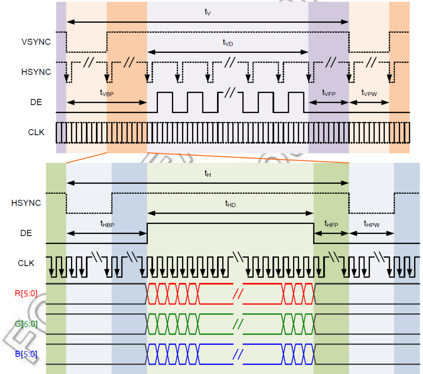
Figure 6.4.1 Data Input Timing Diagram Under DE Mode
