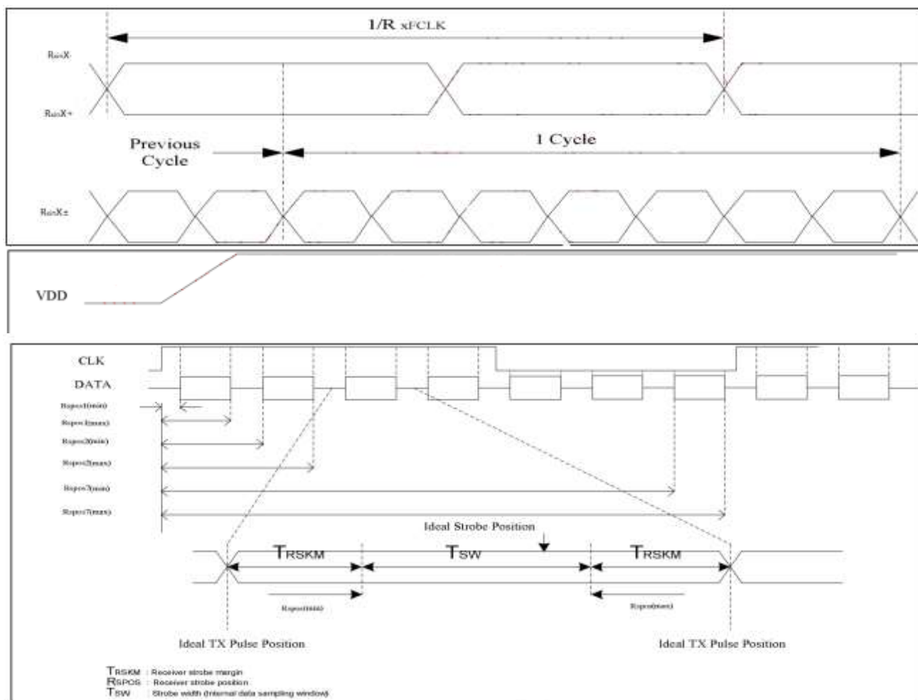
Figure 6.3.2 LVDS AC characteristics
