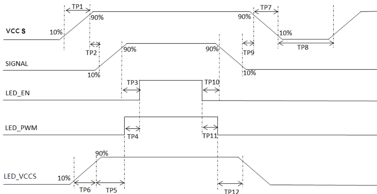
Figure 5.3.2 Power ON/OFF Sequence
