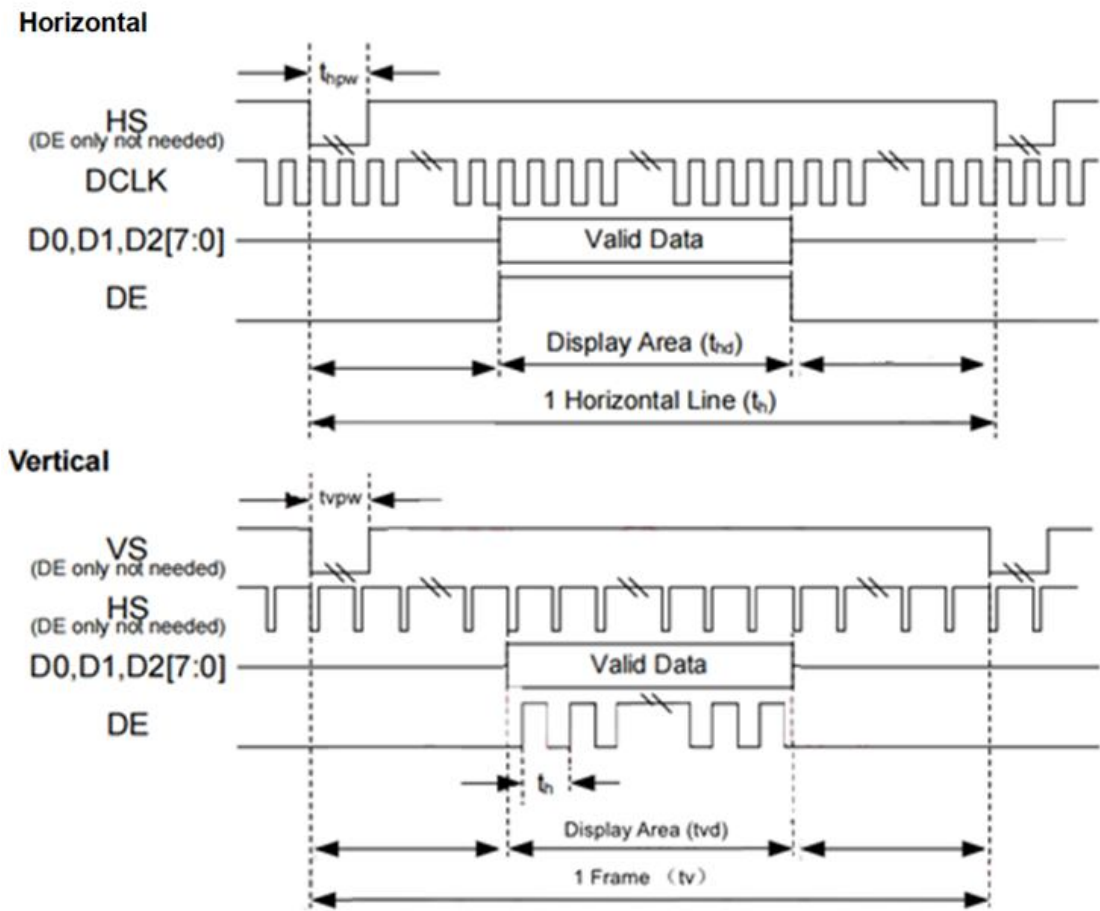
Figure 6.3 Data Input Timing Diagram Under DE Mode
