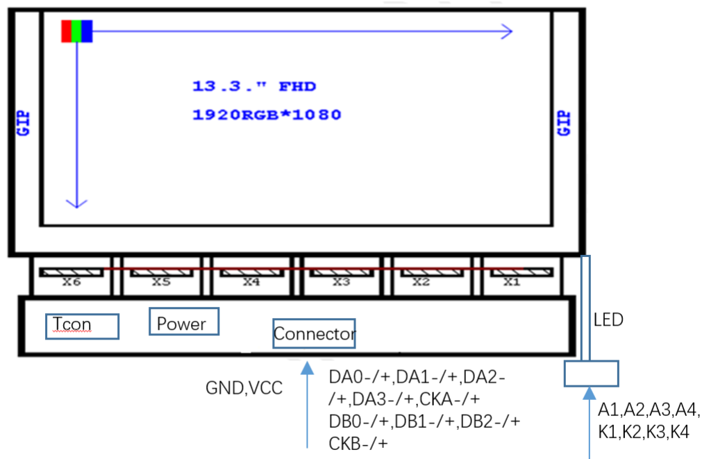
Figure5.3. Block Diagram
