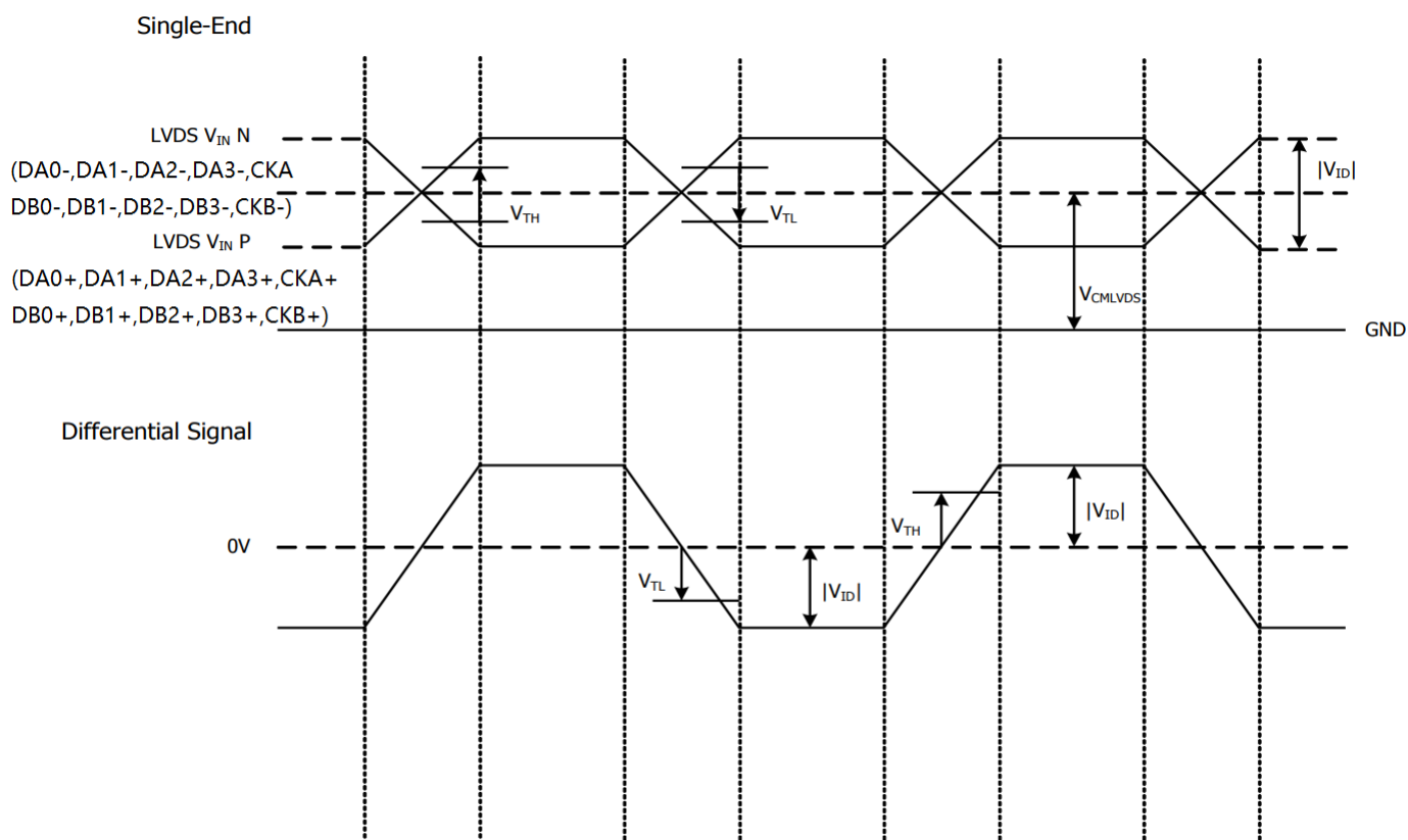
Figure 6.2.1. LVDS Waveform
