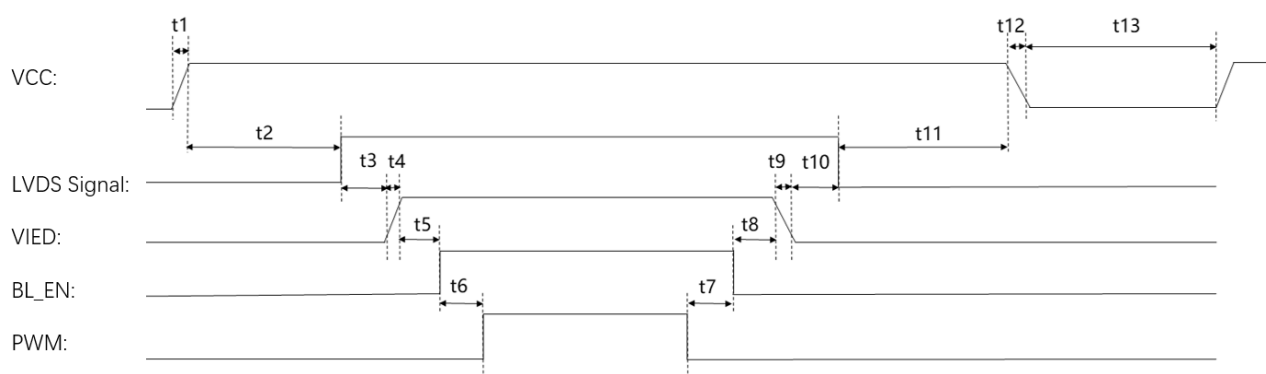
Figure 5.3.1 Power on/off sequence
