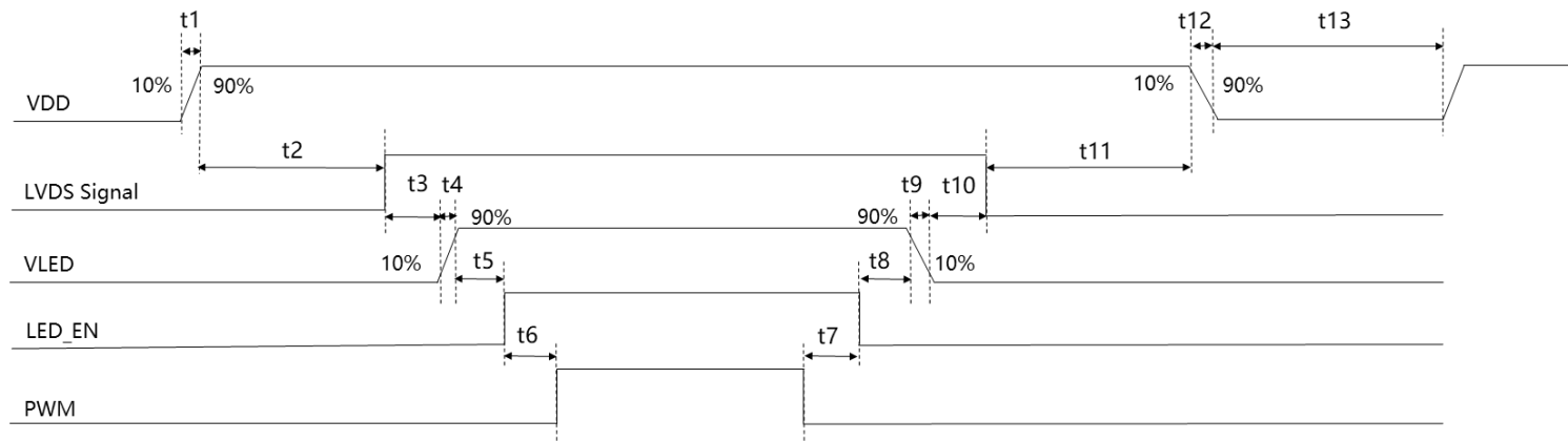
Figure 5.3.1 Power on sequence
