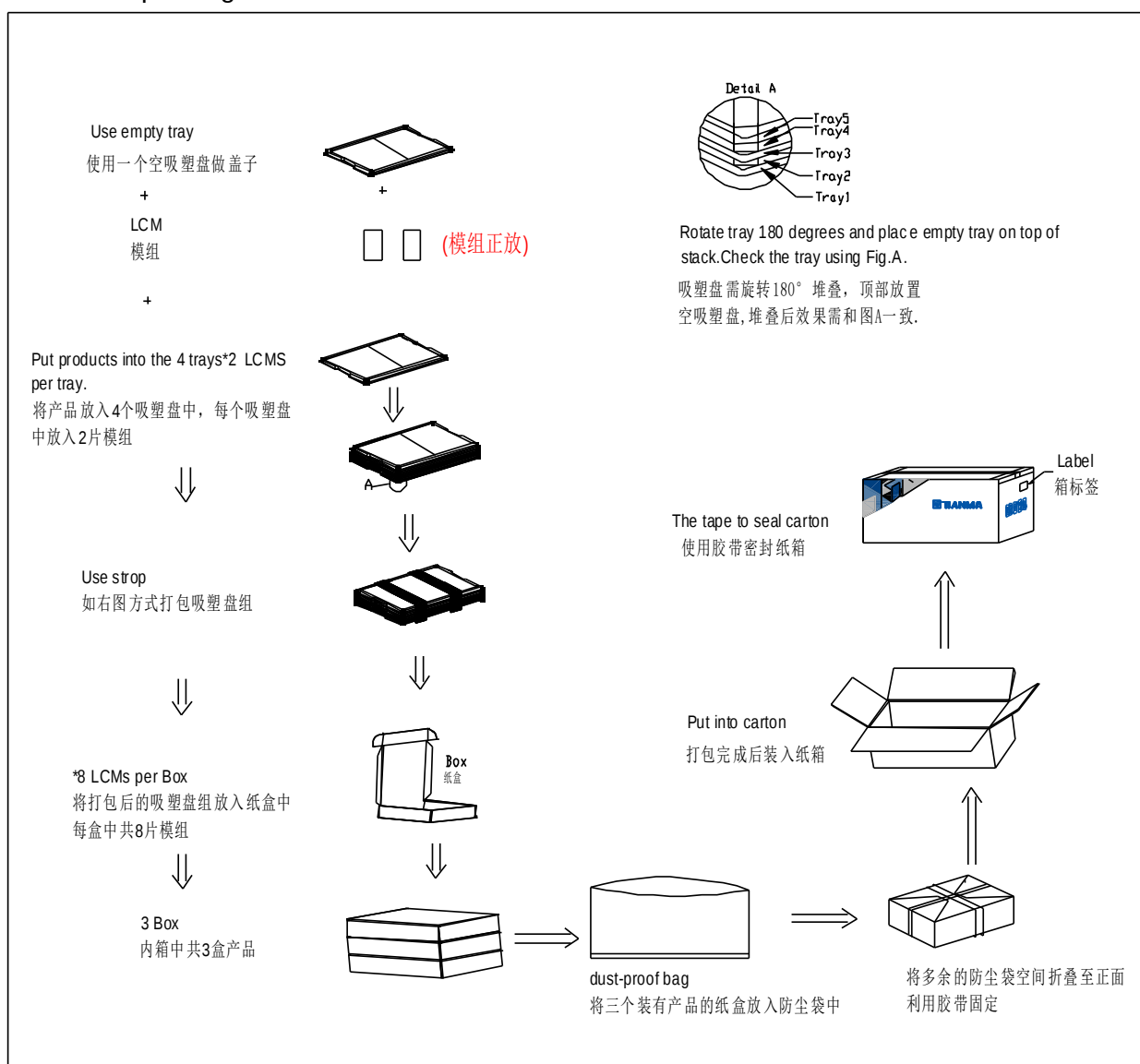
Figure10.1 Packing instruction
