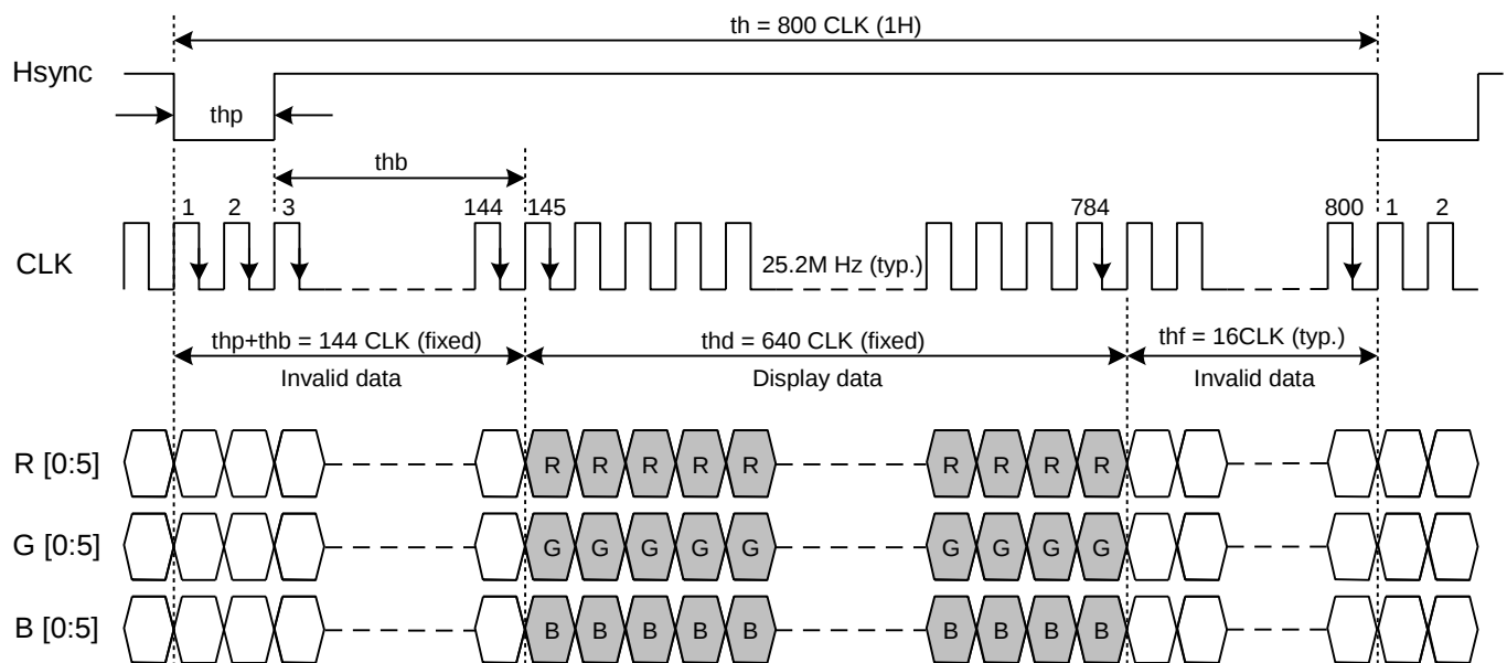
Fig. 9.1 Horizontal Timing
